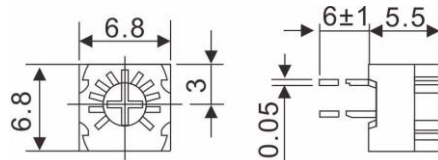
共有尺寸 Common Dimensions
