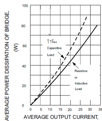
FIG.6-MAXIMUM POWER DISSIPATION
