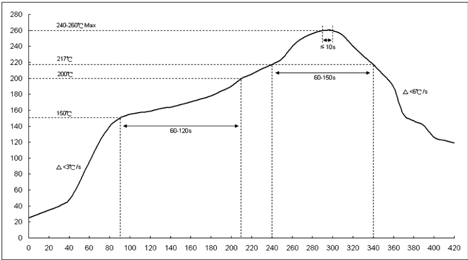
Recommend reflow soldering profile
