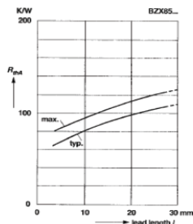
Thermal resistance versus lead length
